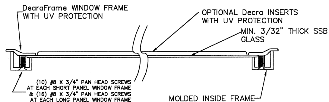
SECTION B-B
